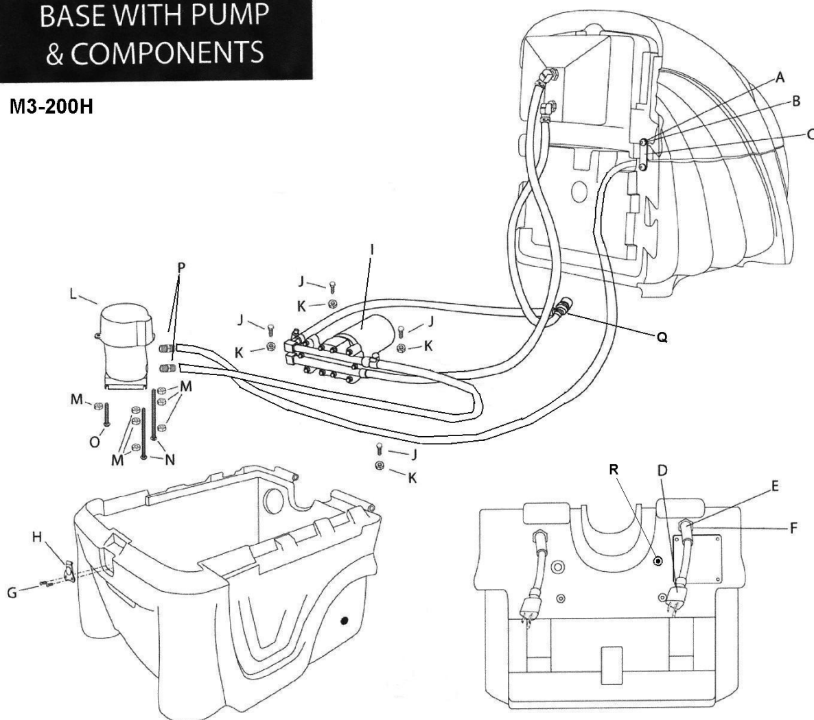
REAR VIEW
