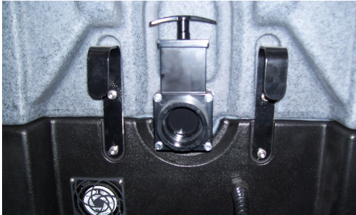
Remove four bolts holding valve assembly to flange fitting
