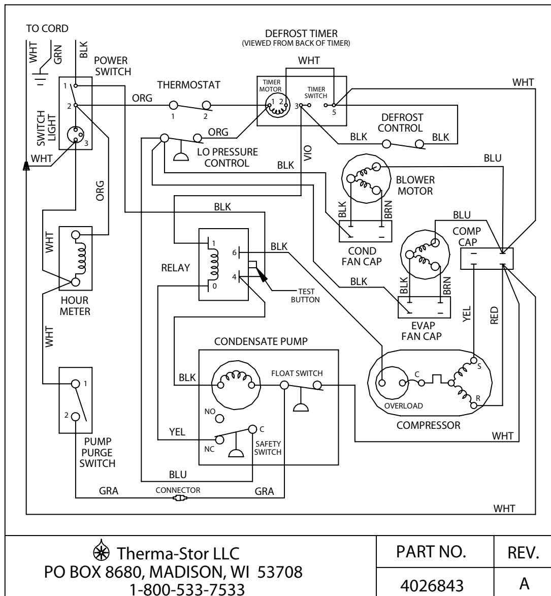
Figure 8: Wiring diagram
