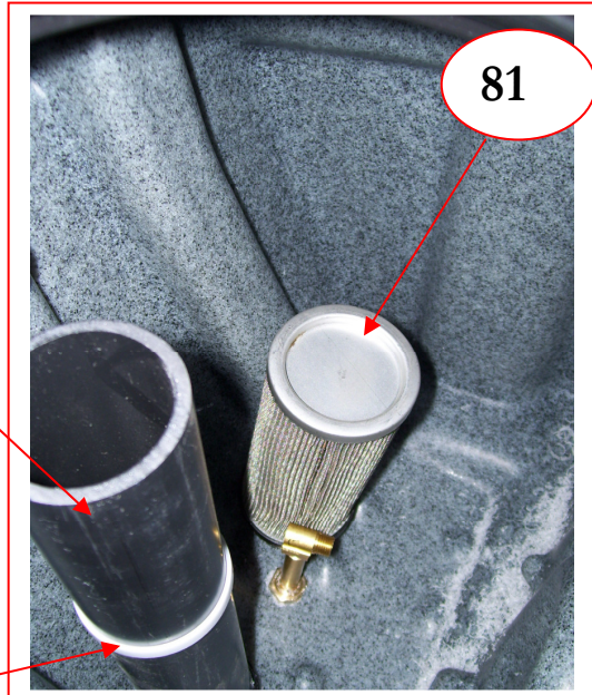
INSIDE RECOVERY TANK WITH OPTIONAL PUMP-OUT FILTER IN PLACE
